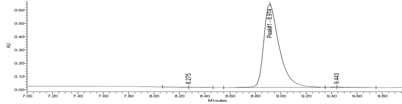
HPLC-UV Chromatogram
