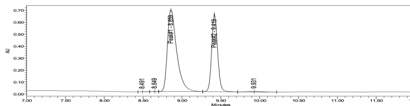
HPLC-UV Chromatogram
