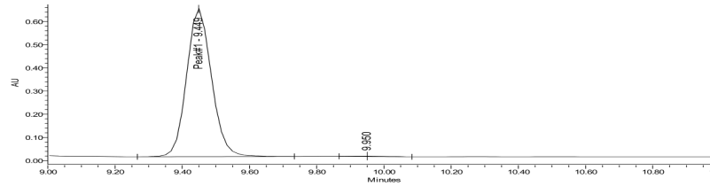
HPLC-UV Chromatogram
